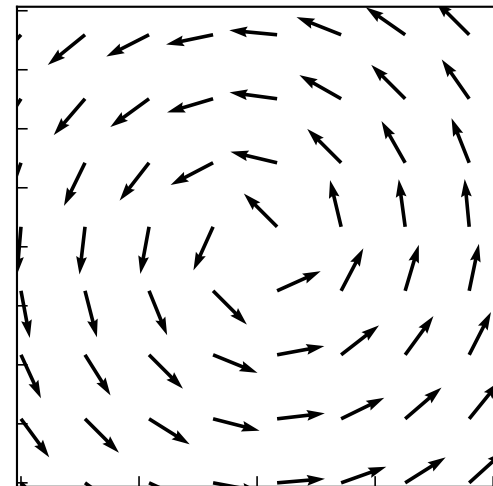
Perp of \nabla f(x, y)
