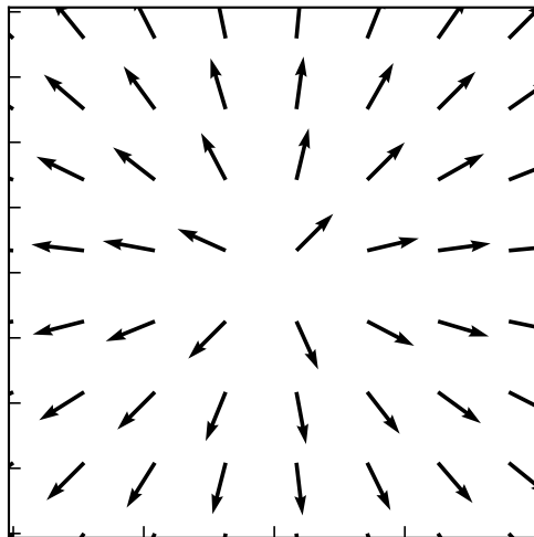
\nabla f(x, y)
